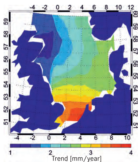
Fig. 2.3: Trend of sea level in the North Sea (April 1993 to December 2012) calculated on the basis of monthly averaged altimeter data. Land elevation and subsidence processes were not taken into account in this investigation. (Graphics: Saskia Esselborn, GFZ)
