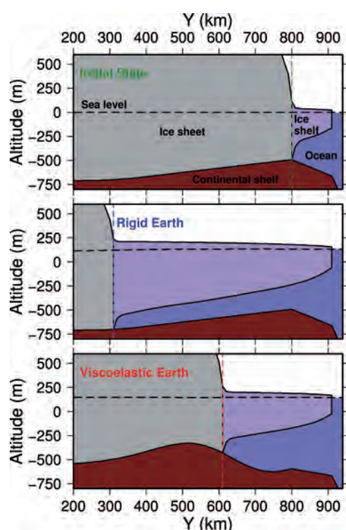
Fig. 2.1: Simulated influence of Earth deformation and change in sea level on the position of the grounding line. Top: initial state. Middle: no Earth deformation, only change in sea level (120 m, similar to after the last ice age). Bottom: Earth deformation and change in sea level. As can be seen, the loss in mass of the ice sheet due to the change in sea level (middle) for the case of deformable Earth leads to a land uplift that contributes to an earlier stabilisation of the grounding line (bottom). (Graphics: Hannes Konrad, GFZ)
