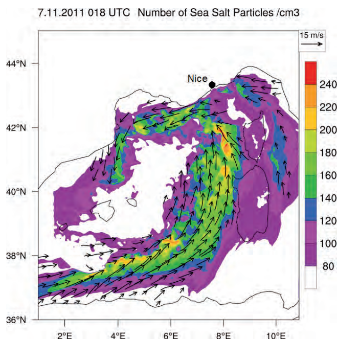
Fig. 1.3: Wind field (vector arrows) and numerical density of sea salt particles (colour coding) for 7 November 2011 at 20 m above sea level at 18:00 UTC. (Graphics: Isabel Kraut, KIT)
