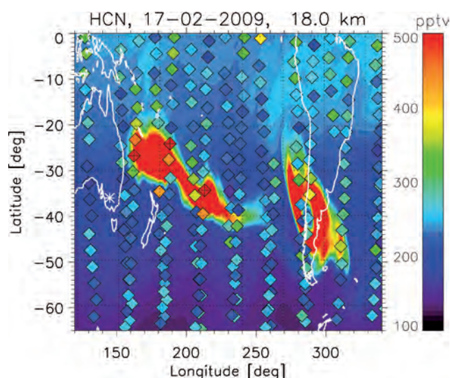
Fig. 5.1: Concentration distribution of hydrocyanic acid from fires in southeast Australia at a height of 18 km (i.e. in the stratosphere) in February 2009. The diamonds represent the MIPAS observations while the coloured areas in the background are model calculations with the GEM-AQ model. (Source: Glatthor et al., 2013)
