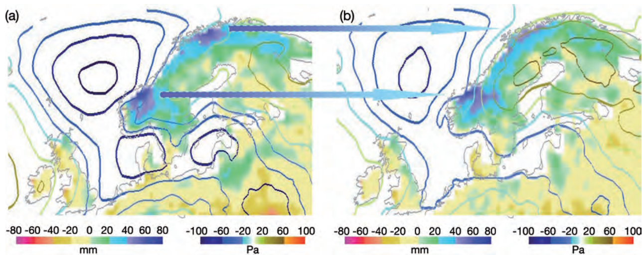
Fig. 1.2: Differences in precipitation (mm/month, colour coding) in comparison to reference data (WATCH) for CCLM (a) and COSTRICE (b). Differences in the reduced sea level pressure (Pa, contours) in comparison to reanalysis data (ERA-Interim). Both averaged over the summer 1998-2002. (Graphics: Ha Hagemann, HZG)
