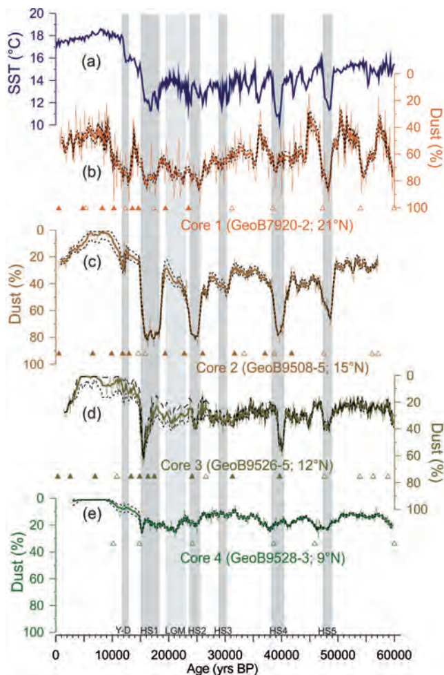
Fig. 8.2. a): Reconstructed sea surface temperature (SST) record of the Iberian margin (Martrat et al., 2007). b – e) Dust content (%) of each of the cores (1–4) from West Africa. Grey bars highlight Heinrich Stadials (HS) 1–5. (Graphics: modified from Collins et al., 2013).
