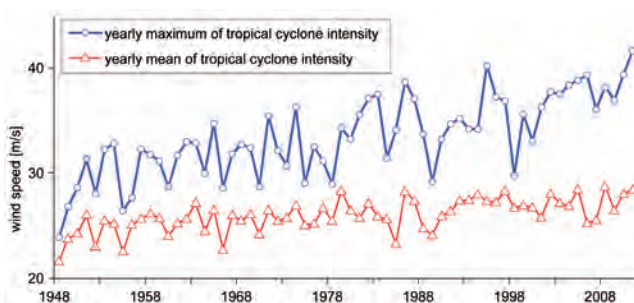
Fig. 6.1: Annual maximum and mean values of the tropical cyclone intensity of all tropical cyclones followed in the CCLM regional model. The intensity is shown as maximum wind speed near the ground. The X axis shows the time in years. (Graphics: Monika Barcikowska, HZG)
