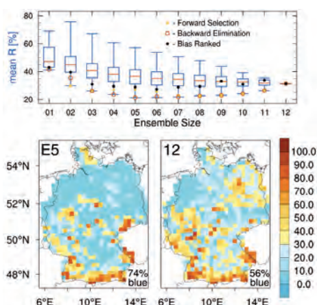
Fig. 6.3: Top: Variability of mean percentage of significant extreme indices (5% significance level) depending on ensemble size (box plots). Furthermore, the “mean R” of the combinations found using different selection methods is shown. Bottom: Spatial variability of the percentage of extreme indices for the best combination of five models that was selected through backward elimination (E5) as well as the ensemble of all models (12). (Graphics: Stephan Thober, UFZ)
