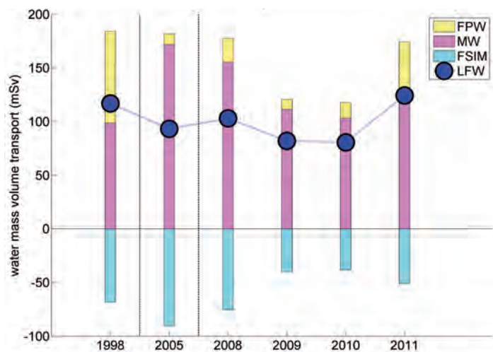
Fig. 3.3: Freshwater transport through the western Fram Strait (11°W to 4°E, red arrow) from temperature, salt concentration, tracer and direct velocity measurements during the respective exposure (positively to the south). Blue circles: total freshwater export relative to 34.9 salt concentration. Transport portions of meteoric water (MW: continental discharge and precipitation) in magenta, Pacific water (FPW) in yellow and net sea ice melt (FSIM) in turquoise. Negative sea ice melt water transport corresponds to southward transport of salt-enriched water from sea ice formation. (Graphics: Benjamin Rabe, AWI).
