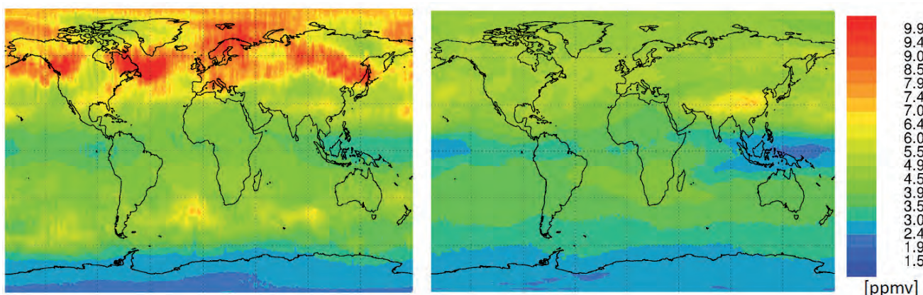
Fig. 5.3: Model simulations of water vapour in the lower stratosphere with two different transport schemes: On the left the results from EMAC with the classic semi-Lagrange scheme, on the right the results with the new coupled trajectory model EMAC-CLaMS. While the water vapour in the classic model is considerably overestimated in the summer hemisphere, initial results of the new model system show lower values here. (Source: Charlotte Hoppe, KIT)
