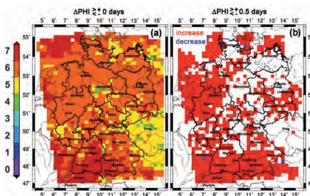
Fig. 6.4: Summary depiction of change in potential hail index PHI between 2021-2050 and 1971-2000 on the basis of an ensemble of seven regional climate simulations: a) number of runs that show an increase, b) only increase or decrease, where red signifies that 5 to 7 models show an increase or 0 to 2 models show a decrease (blue inverse). Here only changes greater than 0.5 PHI in the respective regional run were taken into account. (Graphics: Susanna Mohr und Michael Kunz, 2013)
