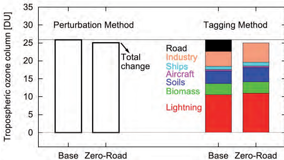
Fig. 5.2: Tropospheric ozone column in Dobson units (DU) for a reference simulation (base) as well as a simulation without road traffic emissions (zero road). Results of the perturbation method are shown on the left and those by means of the tagging method on the right. (Source: Grewe et al., 2012)
