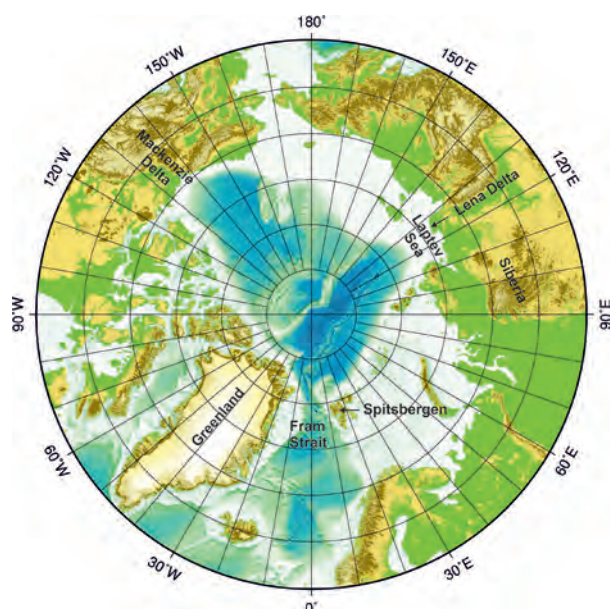
Fig. 3.1: Map with investigation areas designated in the text. (Graphics: Andreas Wisotzki, AWI)
