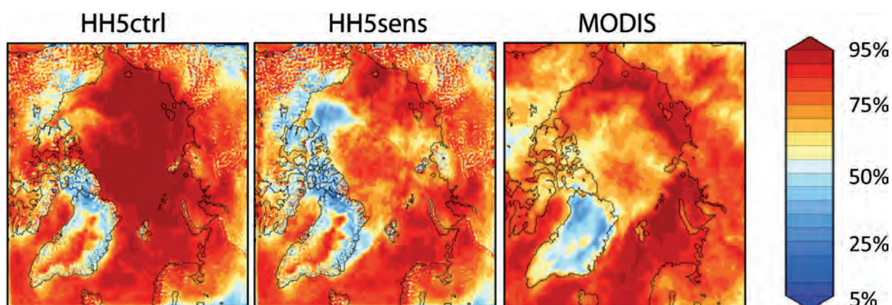
Fig. 1.1: Cloud cover over the Arctic for September 2007 from a control run (HH5ctrl), a sensitivity run (HH5sens) and observations (MODIS). (Graphics: Daniel Klaus, AWI)
