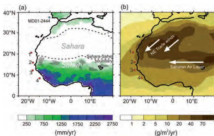
Fig. 8.1. a) Map of West Africa illustrating rainfall distribution (mm/yr). Hatching marks relict sand dunes in the Sahel. Red dots mark core sites (1-4) of our dust records. b) Modern dust deposition (g/m²/yr) illustrating the Saharan dust plume. Modern wind regimes are marked. (Graphics: modified from Collins et al., 2013)
