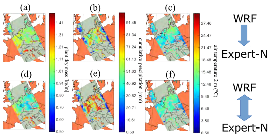
Fig. 4.3: Influence of type of feedback on biomass growth of grassland (illustrations a, d), the cumulative precipitation amounts (illustrations b, e) and the temperatures (illustrations c, f) in September 2010. Illustrations a-c show results of simulations without feedback and illustrations d-f with feedback of the matter fluxes between the land surface model (Expert-N) and the weather model (WRF). (Graphics: Christian Klein, HMGU)
