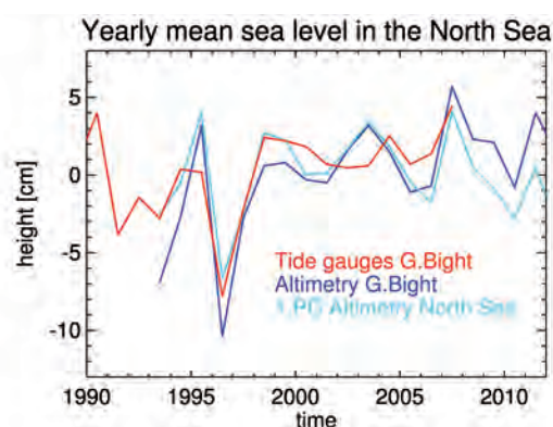
Fig. 2.4: Time series of annual mean of the sea level in the North Sea. Red: amplitude of the first main component from sea level gauge data; blue: mean from satellite altimeter data (Topex, Jason-1/2) for the German Bight in each case; turquoise: amplitude of the first principal component of the altimeter data for the entire North Sea. (Graphics: Frauke Albrechts, HZG; Saskia Esselborn, GFZ)
