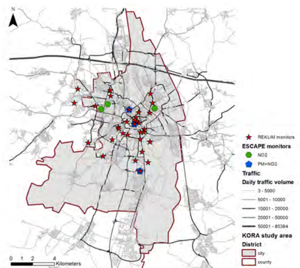
Fig. 9.1: Distribution of REKLIM measurement sites over the city of Augsburg (as of 31 May 2013). (Source: A. Peters, A. Schneider, S. Breitner, T. Kusch, C. Hald, J. Cyrus, HMGU)
