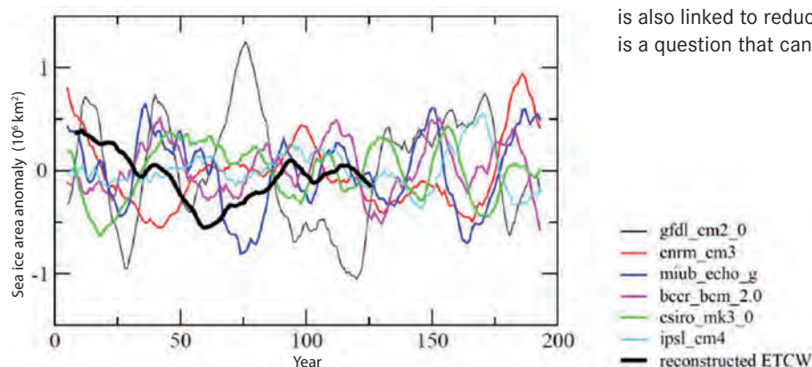
Fig. 3.2: Anomalies of the extent of Arctic sea ice ( 10^6 \text{ km}^2 ) in winter simulated with several climate models (coloured lines) and reconstructed for the period 1880 to 2008 using observed atmospheric temperatures (thick black line). The minimum of the reconstructed anomaly coincides with the maximum temperature of the ETCW. The legend contains the names of the models used. (Graphics: Vladimir Semenov, GEOMAR)
